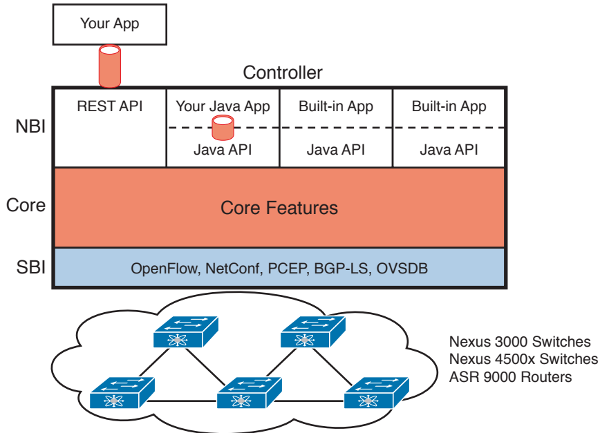
Figure 28-8 Architecture of NBI, Controller Internals, and SBI to Network Devices
