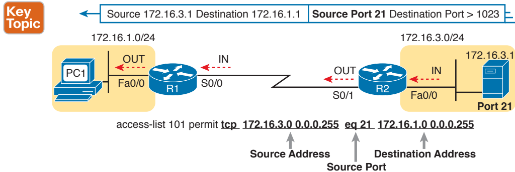
Figure 17-7 Filtering Packets Based on Source Port
