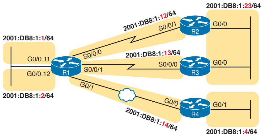
Figure 23-4 Internetwork for an Example Multiarea OSPFv3 Configuration
