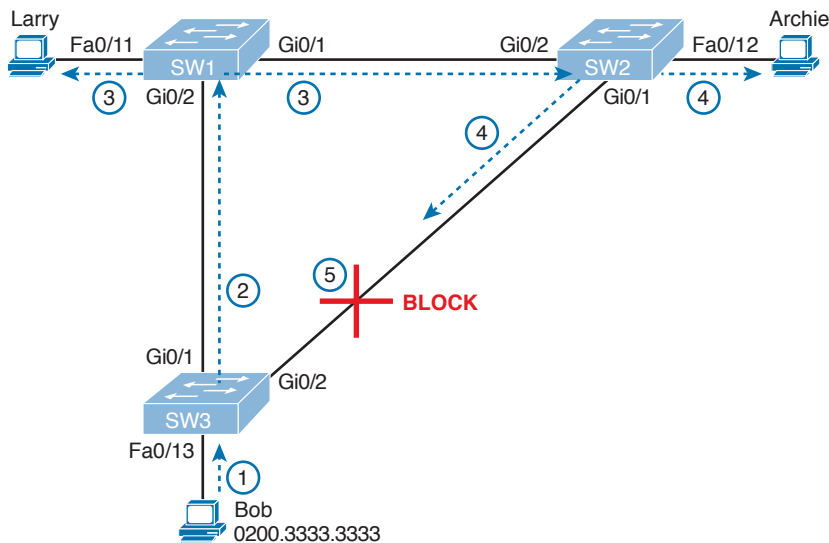
Figure 2-2 What STP Does: Blocks a Port to Break the Loop
