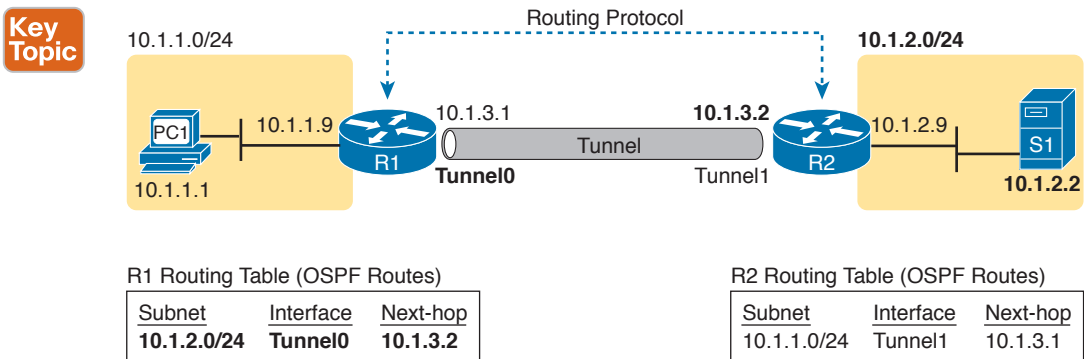
Figure 15-10 Routes Learned with a Routing Protocol over the IP Tunnel
